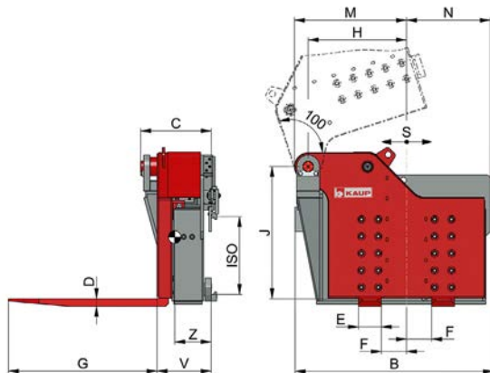
Ladle Tipper T360 - tilt angle \alpha = 100^\circ to the right side in driving direction
