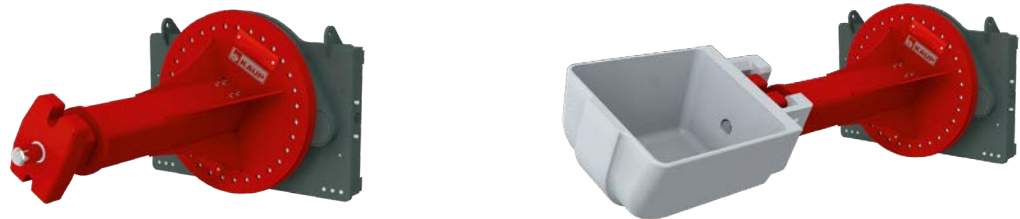
Charging Devices T355 and T395 (with sideshift) in various capacities and versions (upon request).
